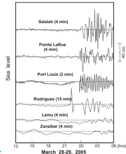
Sumatra Earthquake of March 28, 2005 ( M = 8.7 ) West Indian Ocean
